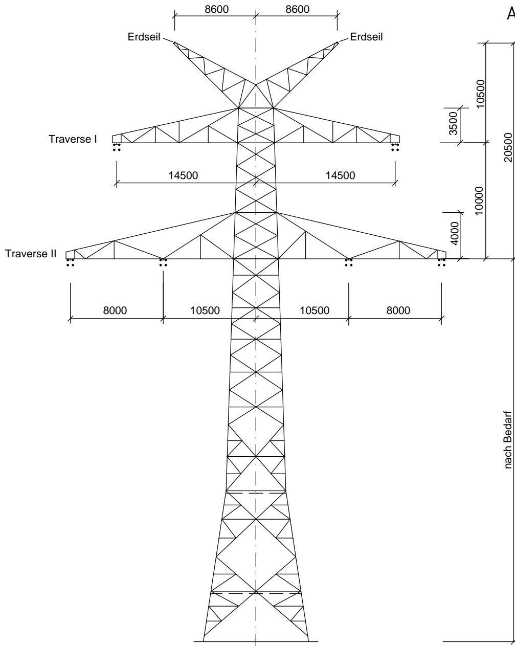
Winkelabspannmast WA100; D-2-D-2015.3 Ltg. Nr. 315; Mast-Nr. 3
