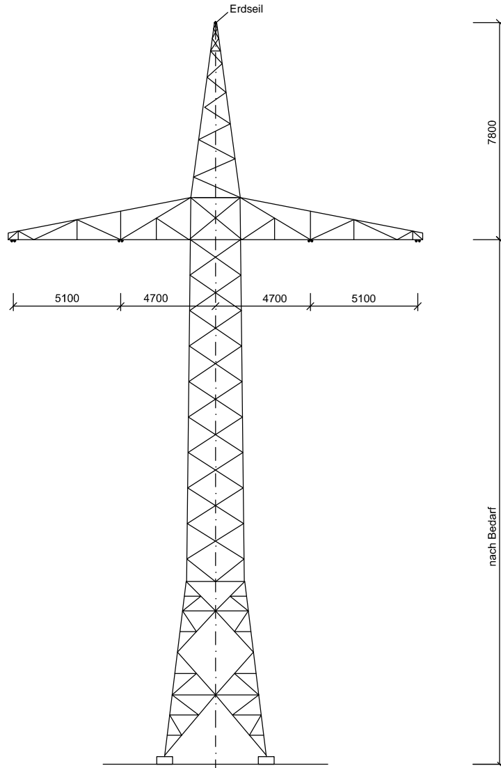
Winklendmast A/E19...100° Ebf 23900 Mast-Nr. 9635N, 9571N (L0564)
