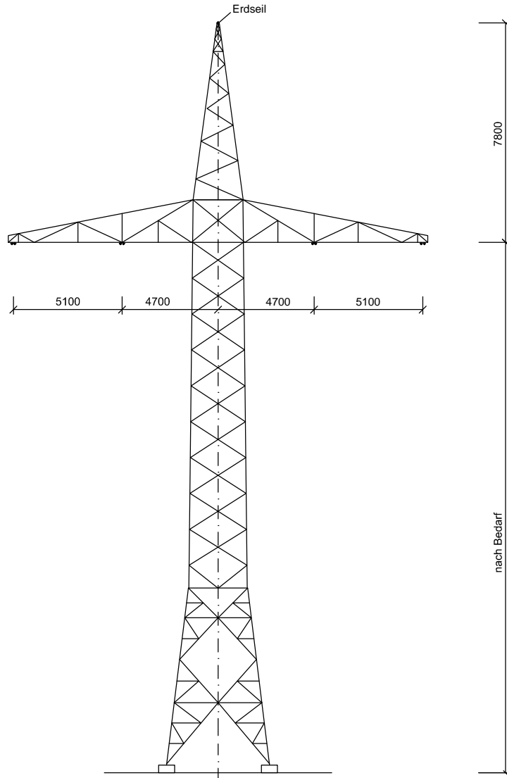
Winkelendmast A/E28...100° Ebf 23900 Mast-Nr. 9642N, 9607N (L0564)
