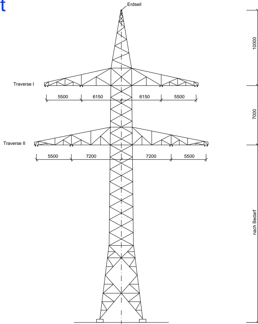
Winkelendmast A/E16...100° Ebf 24512 Mast-Nr. 9665N (L0564, L0457)
