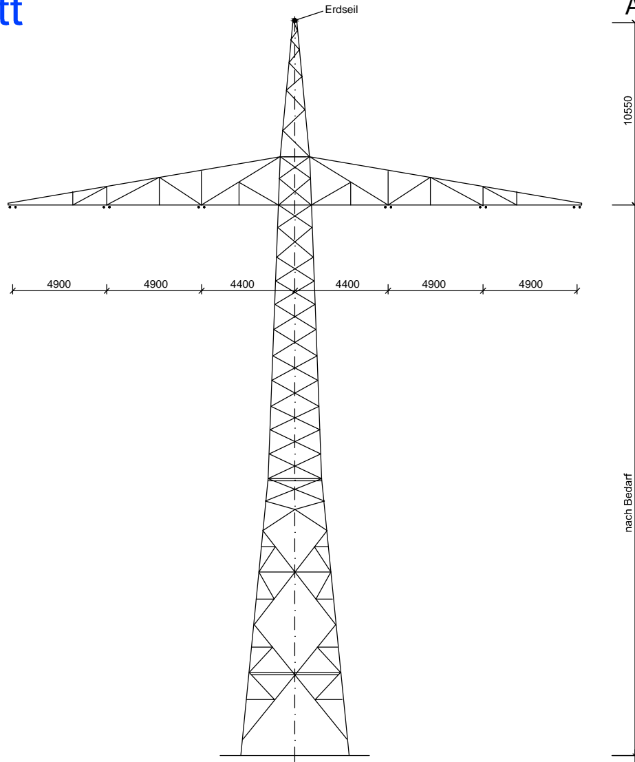
Winkelendmast WE100; A-2-E-2007.1 Mast-Nr. 023 Bestandsmast (LH-11-1008)
