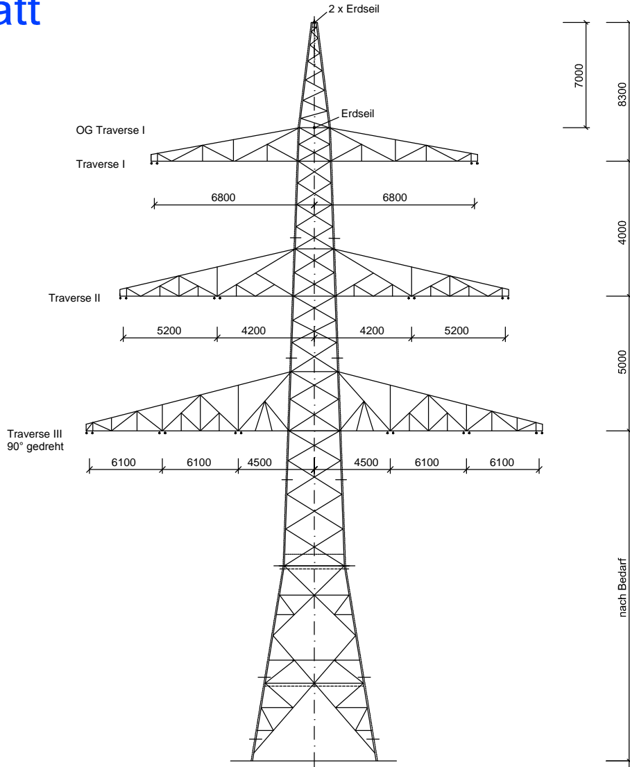
Winkelabspannmast WAZ 120; A-2-D-2013.1 Mast-Nr. 020 (LH-11-1008)
