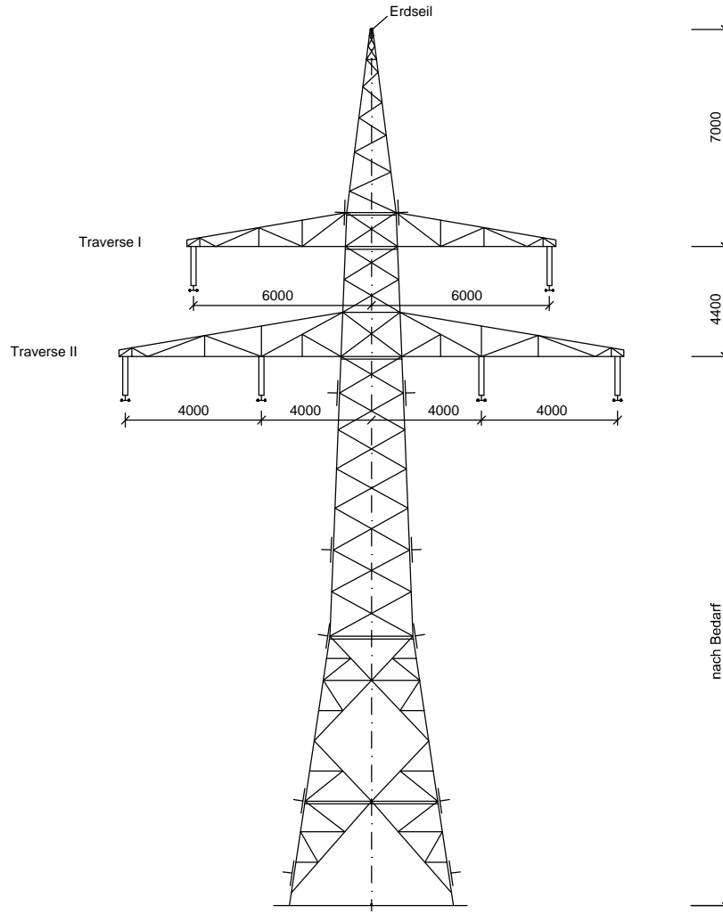
Tragmast T1; A-2-D-2013.1 Mast-Nr. 004, 005, 009, 011, 012, 013, 016, 017, 018, 022 (LH-11-1008)
