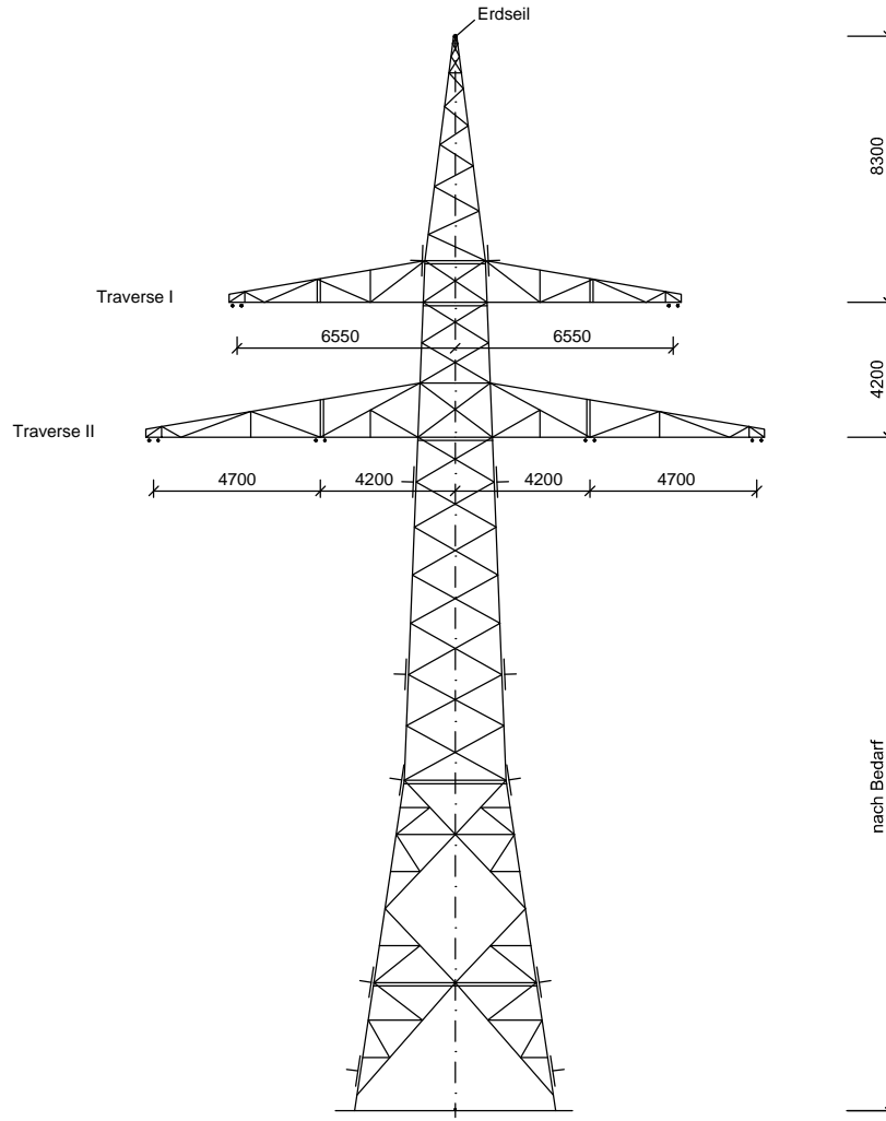
Winkelabspannmast WA 140; A-2-D-2013.1 Mast-Nr. 002, 003, 019 (LH-11-1008)
