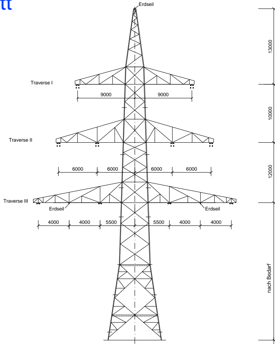
Winkelabspannmast WA 160; DA-4-DE-2013.5 Mast-Nr. C088, C104, C108
