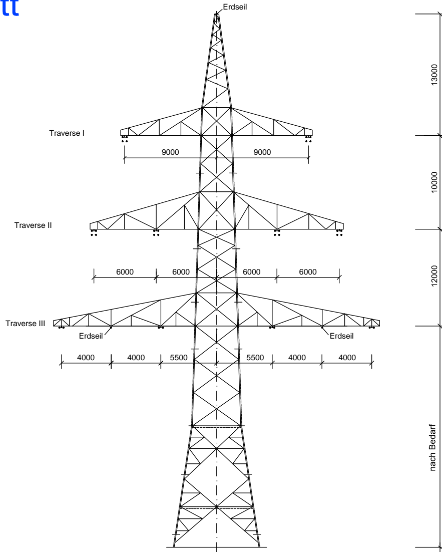
Winkelabspannmast WA 160; DA-4-DE-2015.2 Mast-Nr. C085
