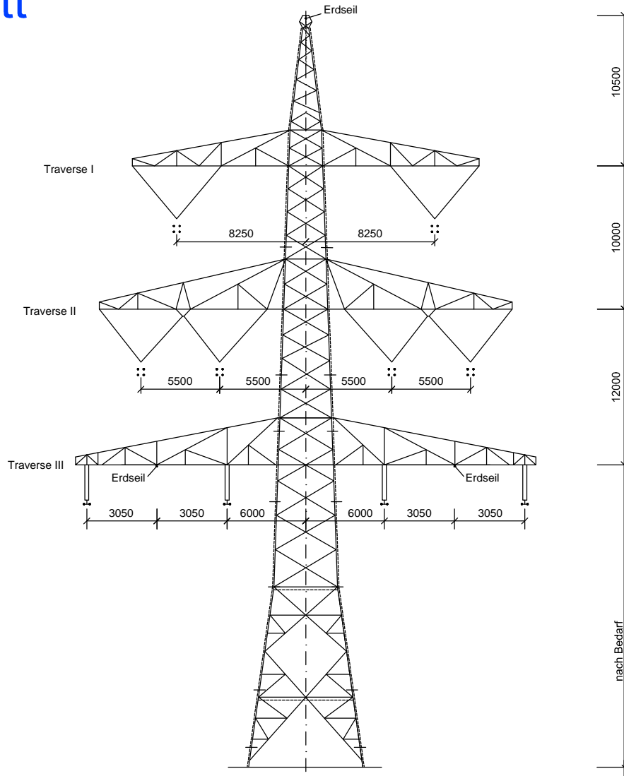
Tragmast T1; DA-4-DE-2015.2 Mast-Nr. C084
