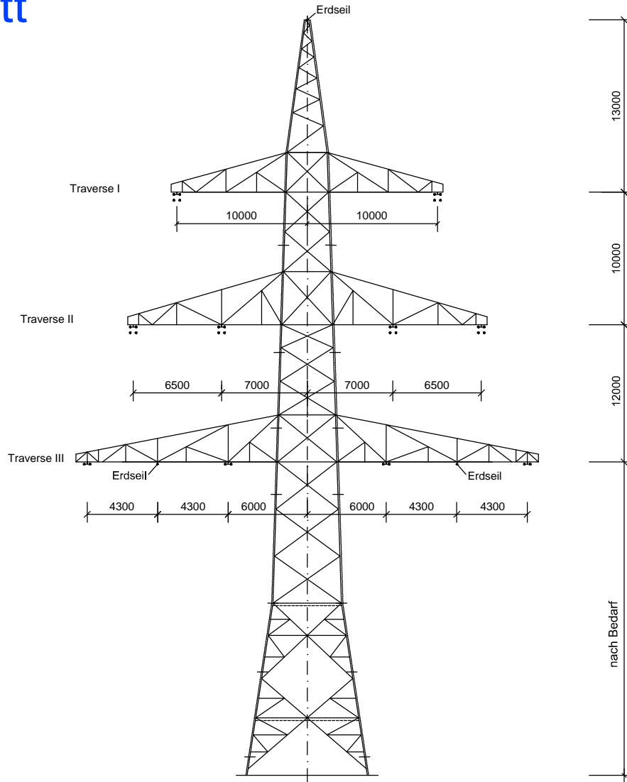
Winkelabspannmast WA 140; DA-4-DE-2015.2 Mast-Nr. C083
