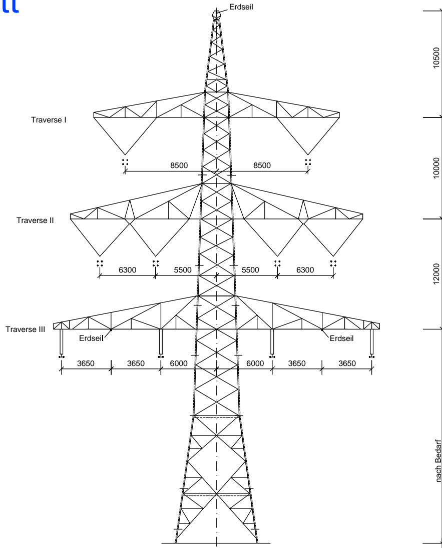
Tragmast T2; DA-4-DE-2015.2 Mast-Nr. C082
