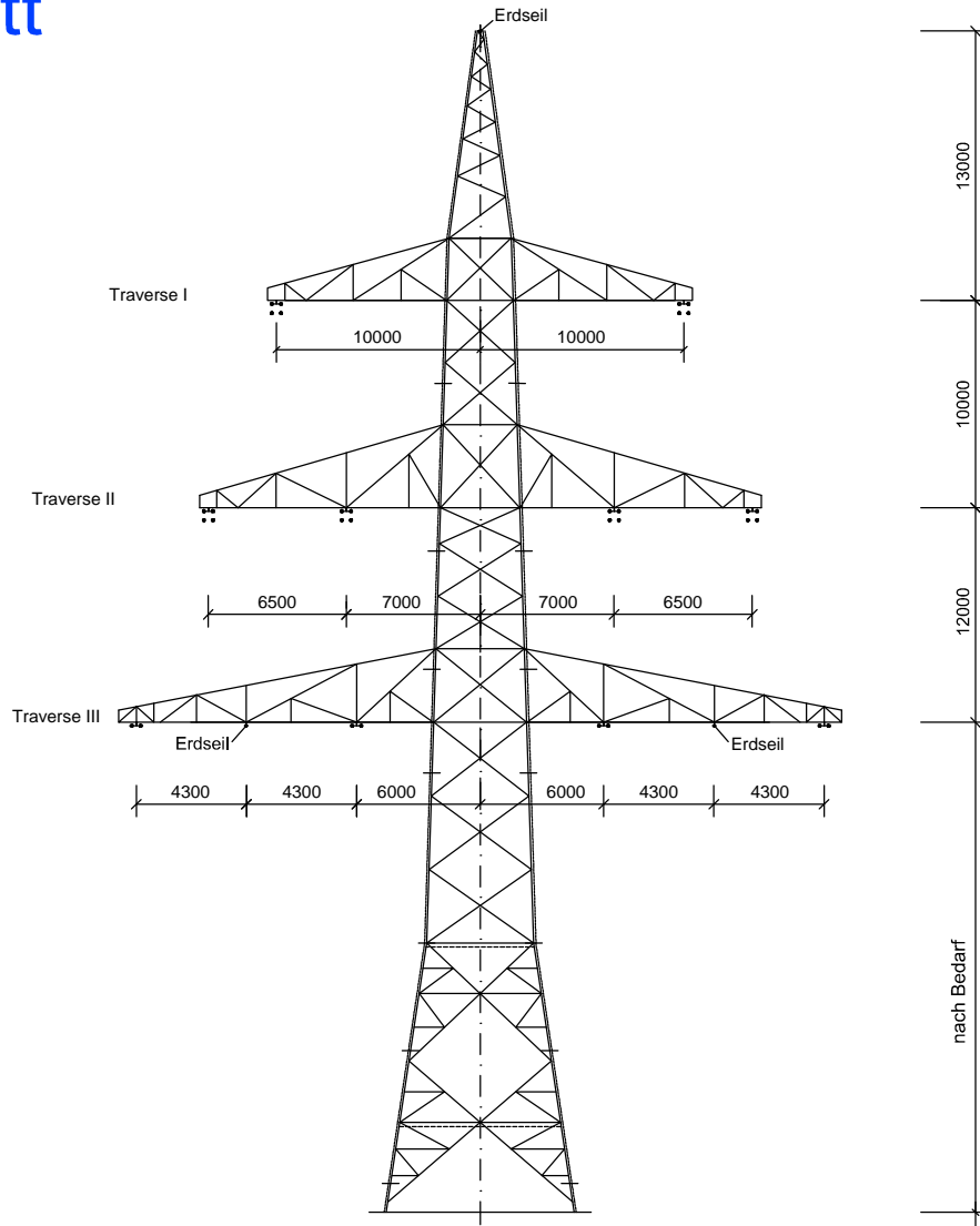
Winkelabspannmast WA 140; DA-4-DE-2013.5 Mast-Nr. C080, C089, C102, C111
