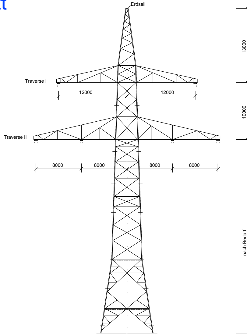
Winkelabspannmast WA 100; D-2-D-2013.1 Mast-Nr. C077
