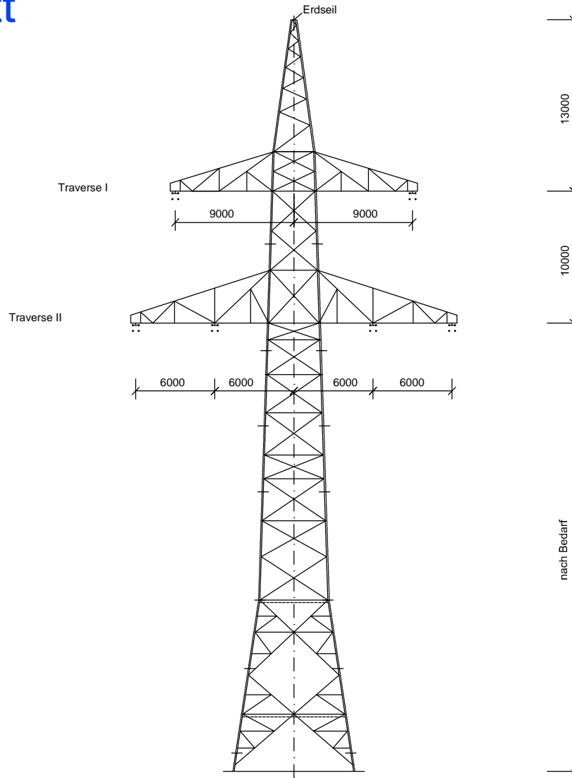
Winkelabspannmast WA 160; D-2-D-2013.1 Mast-Nr. C055, C112
