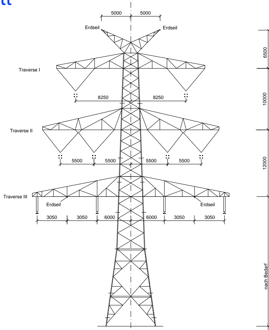
Tragmast T1; DA-4-DE-2015.2 Mast-Nr. C046
