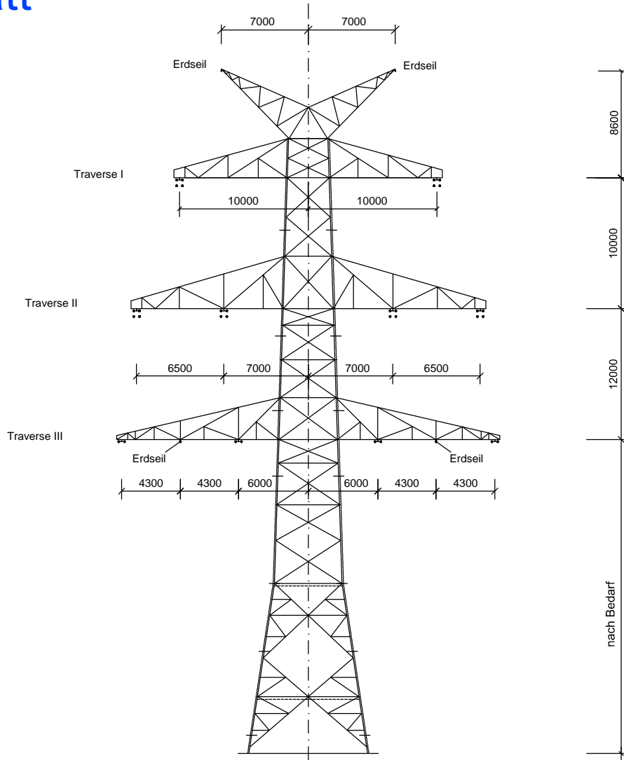
Winkelabspannmast WA 140; DA-4-DE-2013.5 Mast-Nr. C042, C047
