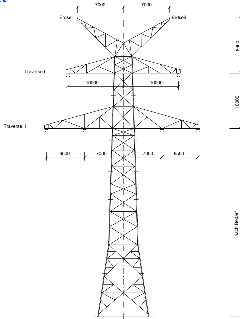
Winkelabspannmast WE/WAdiff 140; D-2-D-2013.1 Mast-Nr. C041
