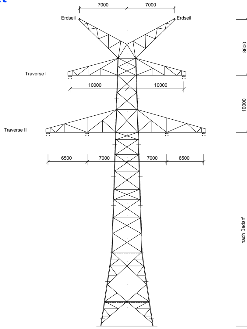
Winkelabspannmast WA 140; D-2-D-2013.1 Mast-Nr. C029
