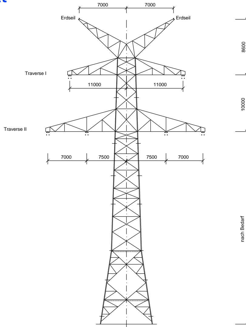
Winkelabspannmast WA 120; D-2-D-2013.1 Mast-Nr. C028
