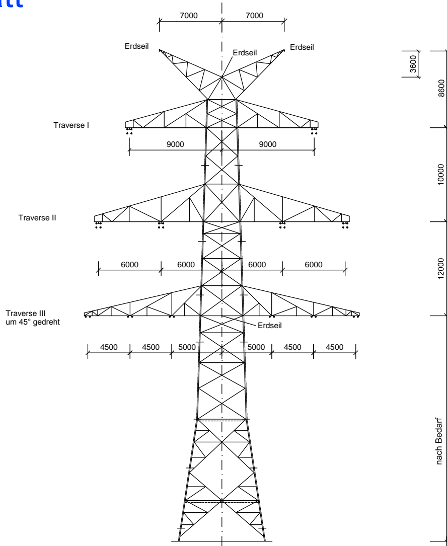
Winkelabspannmast WA 160; DA-4-DE-2013.4 Mast-Nr. C027
