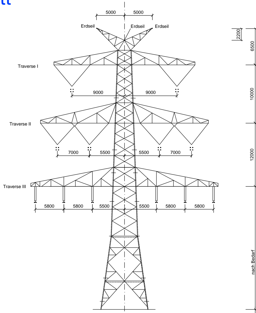
Tragmast T2-spez.; DA-4-DE-2013.4 Mast-Nr. C012
