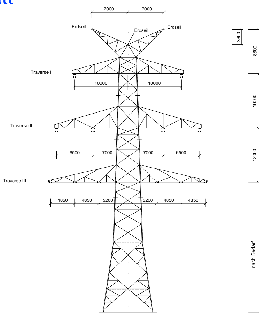
Winkelabspannmast WA 140; DA-4-DE-2013.4 Mast-Nr. C005, C009, C011, C017
