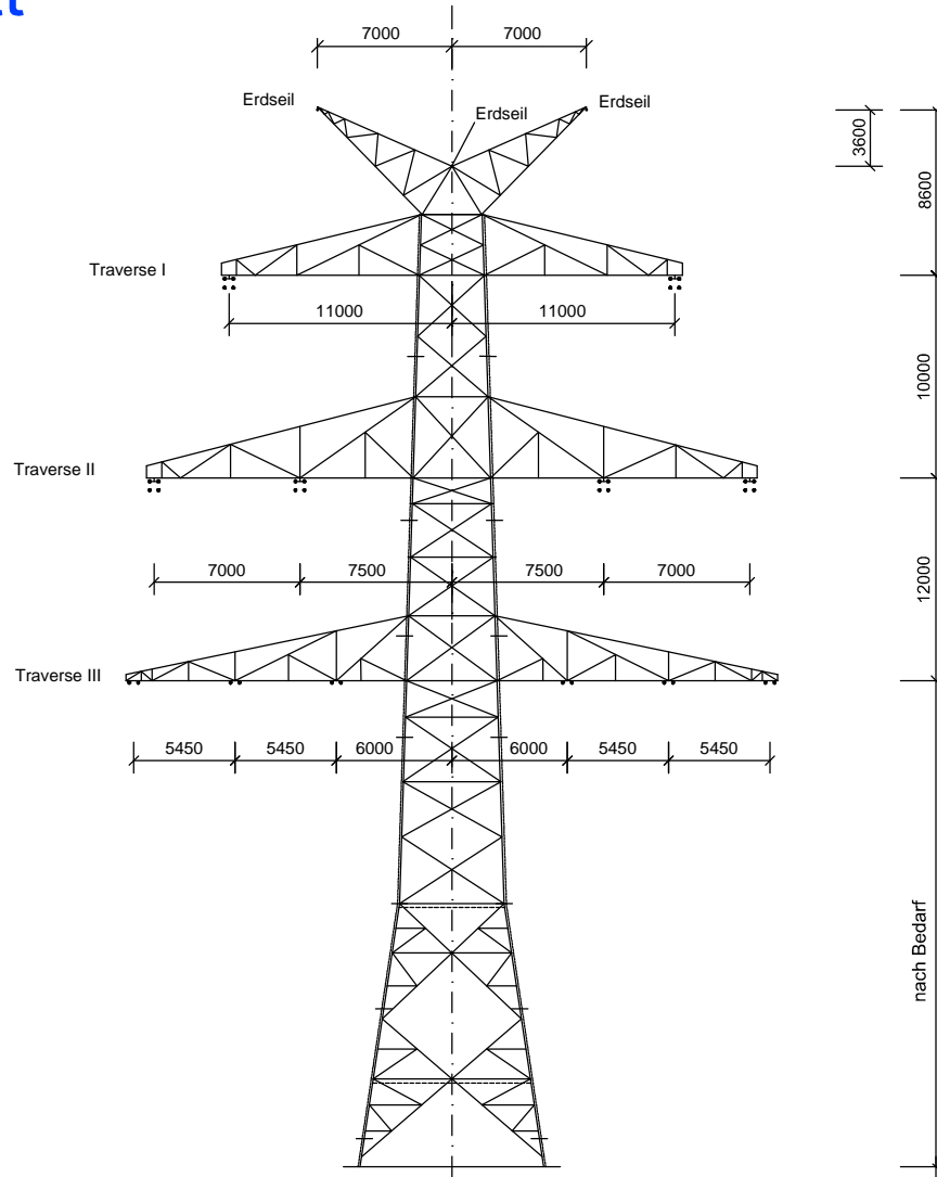
Winkelabspannmast WA 120; DA-4-DE-2013.4 Mast-Nr. C003
