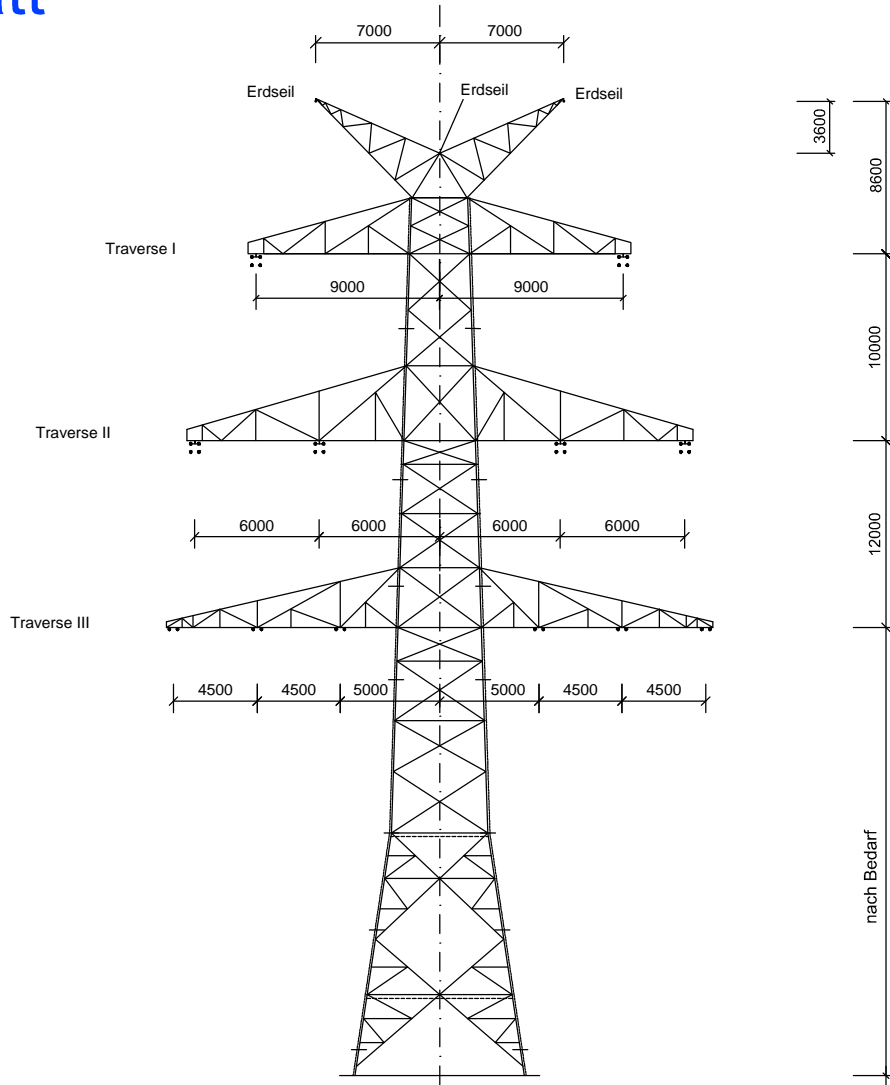
Winkelabspannmast WA 160; DA-4-DE-2013.4 Mast-Nr. C002, C007, C013, C014, C015, C018, C023
