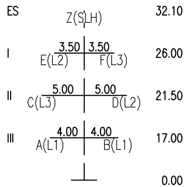
Mast 45
